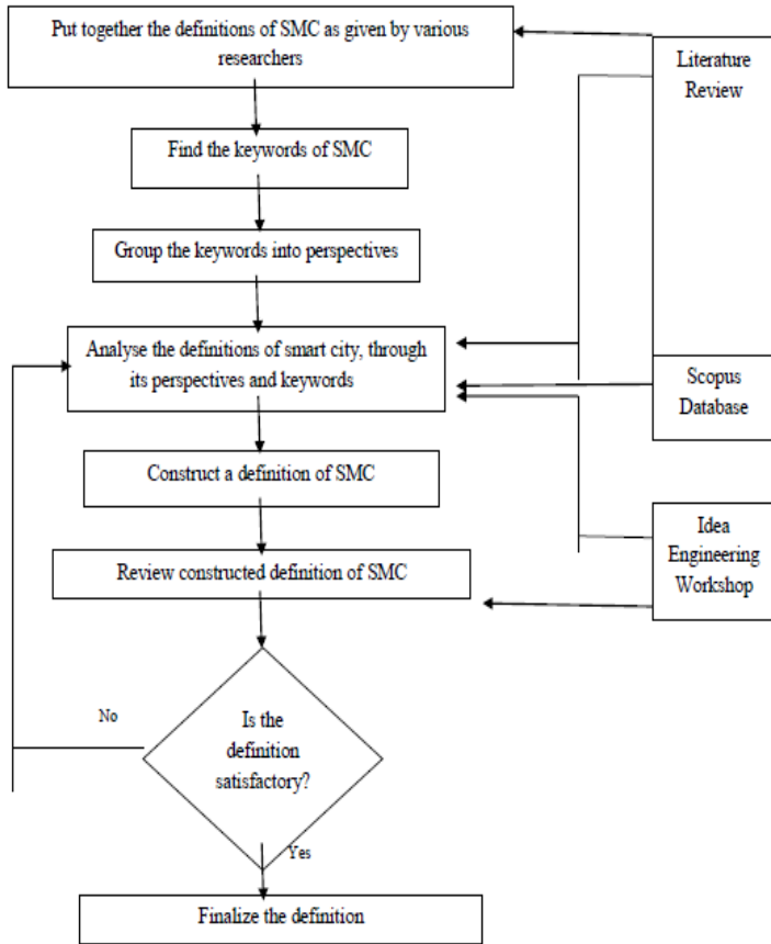
Fig. 1: Methodology Flowchart
